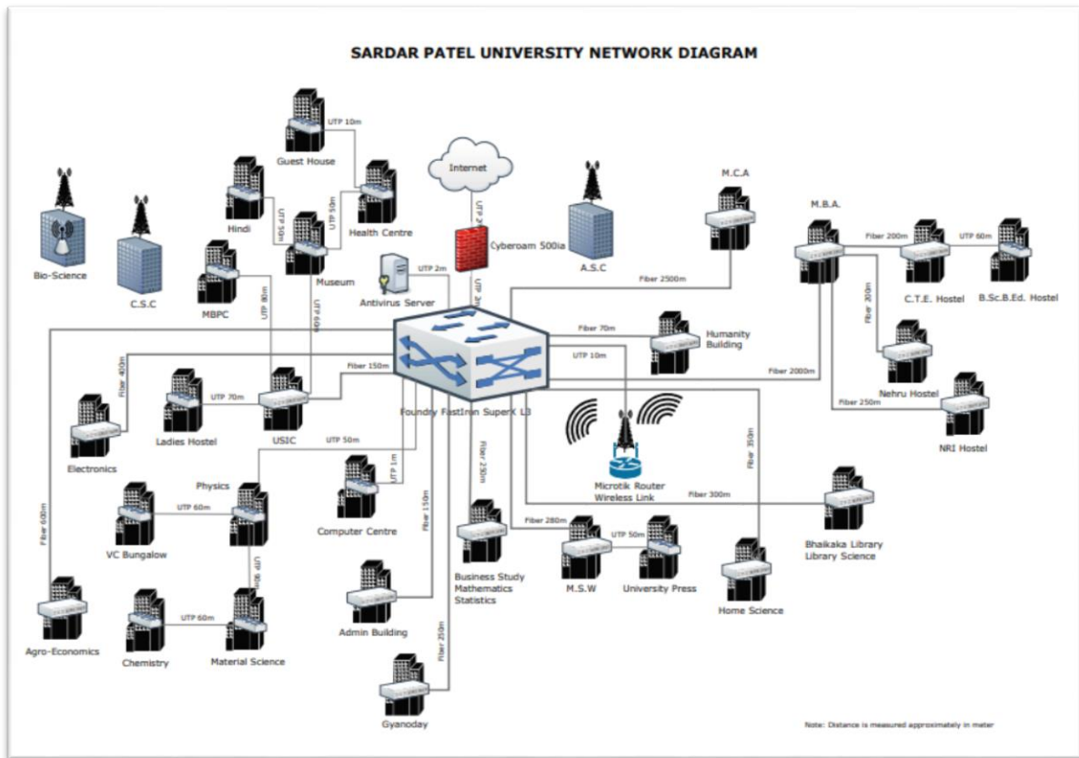
Sardar Patel University Network Diagram
