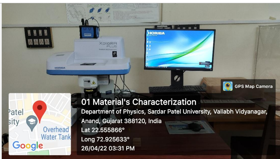
Micro Raman Spectrometer (Horiba Xplora) DST –FIST
