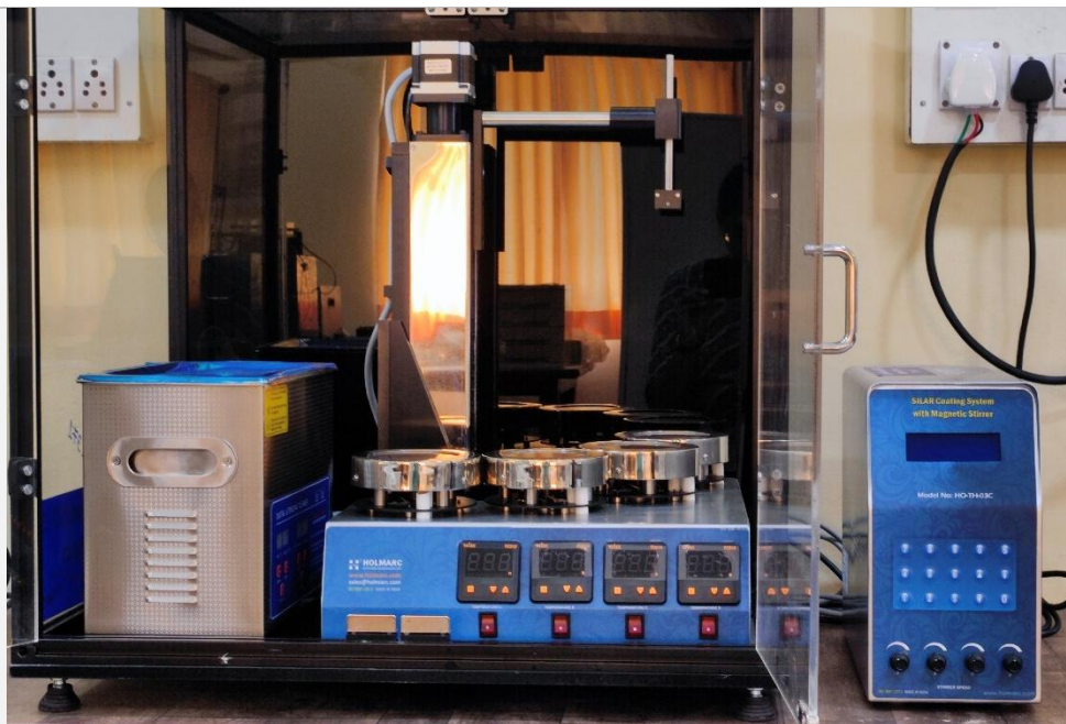
Silar Coating System (HolMarc Opto Mechatronic Ltd) C.C.Desai Mem. Fund
