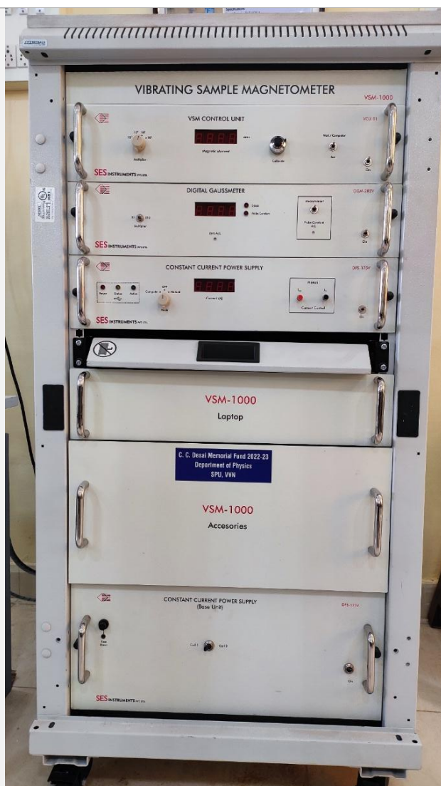
Vibrating Sample Magnetometer (SES Instruments Pvt. Ltd) C.C.Desai Mem. Fund
