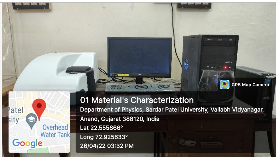
Particle Size Analyser (Malvern Instruments) DRS/SAP
